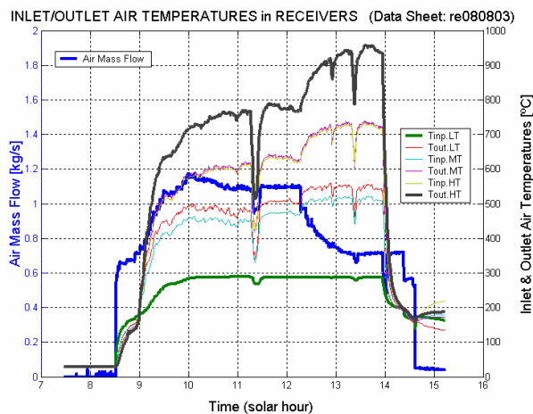
Fig. 21: Air temperatures in the receiver modules..
