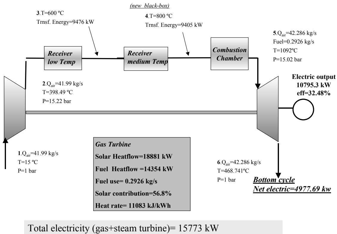
Fig. 33: PGT10 plant. Two receivers configuration scheme
